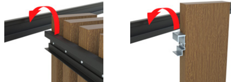
RAIL FASTENING
